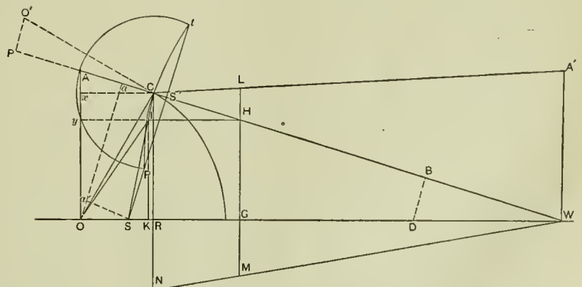
FIG. 5.—CONNECTING ROD THROU DIAGRAM.
